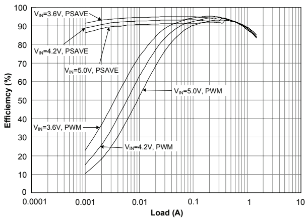
Efficiency vs. Load Current V_{OUT} = 3V
