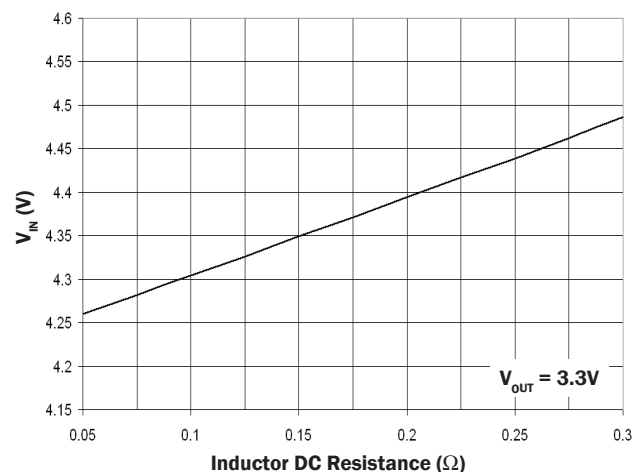
Minimum V_{IN} for Fixed Frequency Operation Vs. R_{IND}
