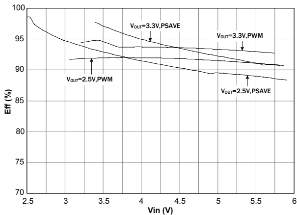
Efficiency vs. Input Voltage V_{OUT} = 3.3V
